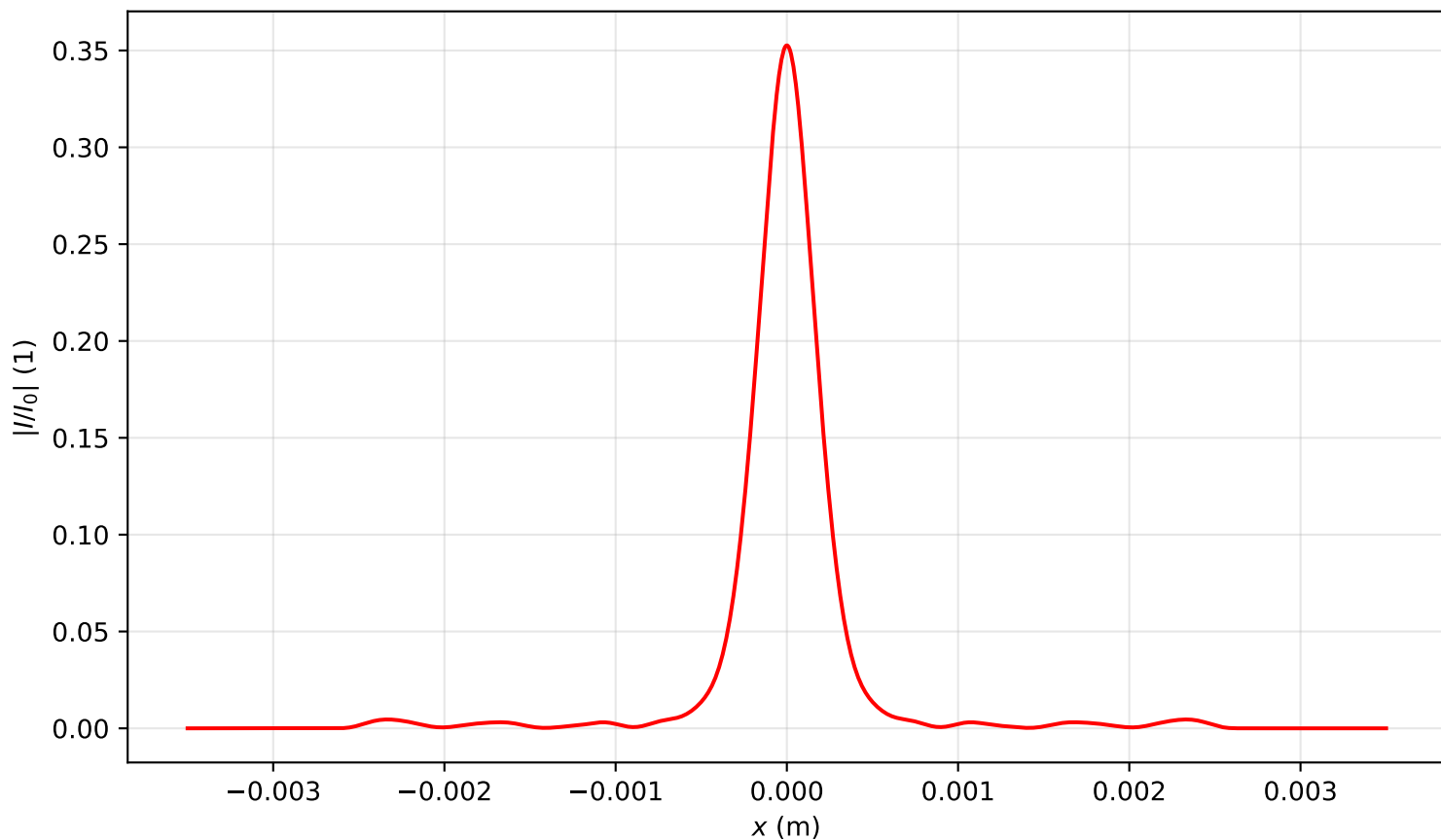
Intensity profile I(x, y = 0, z = 3.662)/I_0 , P_{in}=7.0P_{cr} , artificial time
